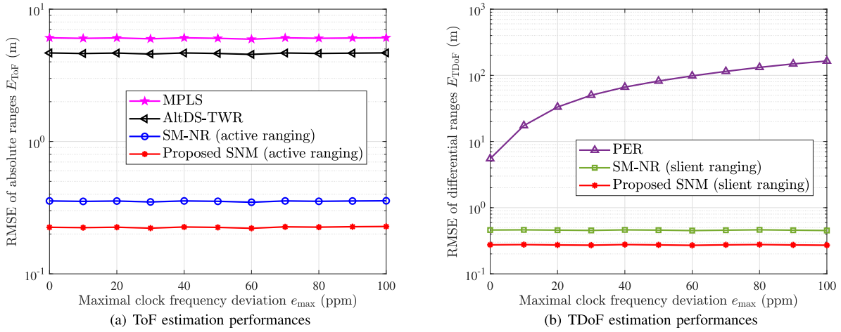
Fig. 7. The RMSEs of (a) absolute ranges; (b) differential ranges against the maximal clock frequency deviation e_{\max} .
