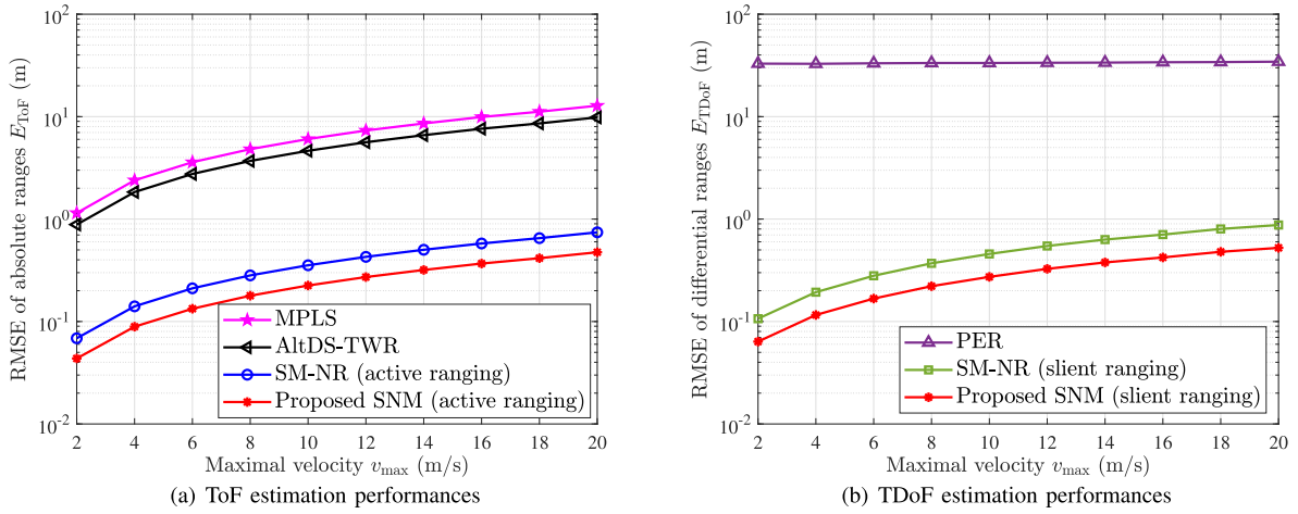
Fig. 6. The root mean square errors (RMSEs) of (a) absolute ranges and (b) differential ranges against the maximal velocity v_{\max} .
