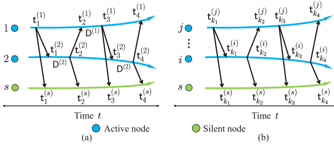
Fig. 3. Illustration of the timestamps captured by SNM, where the curved lines depict that the timestamps are influenced by both time-varying distances and clock drifts.
