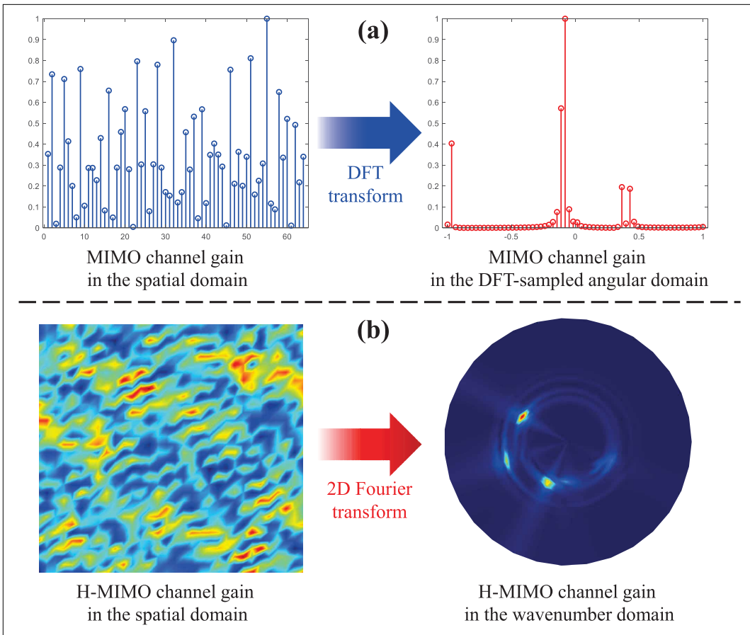
FIGURE 2. a) The channel gains of a 64-antenna MIMO in the spatial domain and the DFT-sampled angular domain. b) The channel gains of a continuous-aperture H-MIMO in the spatial domain and the wavenumber domain.
