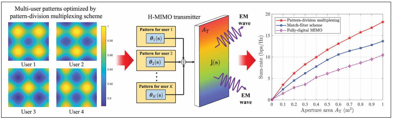
FIGURE 5. An illustration of multi-user H-MIMO downlink transmissions [8]. The multi-user patterns are designed by PDM scheme for sum-rate maximization. Then, the optimized patterns are deployed on the holographic surface of H-MIMO transmitter to serve multiple receivers.
