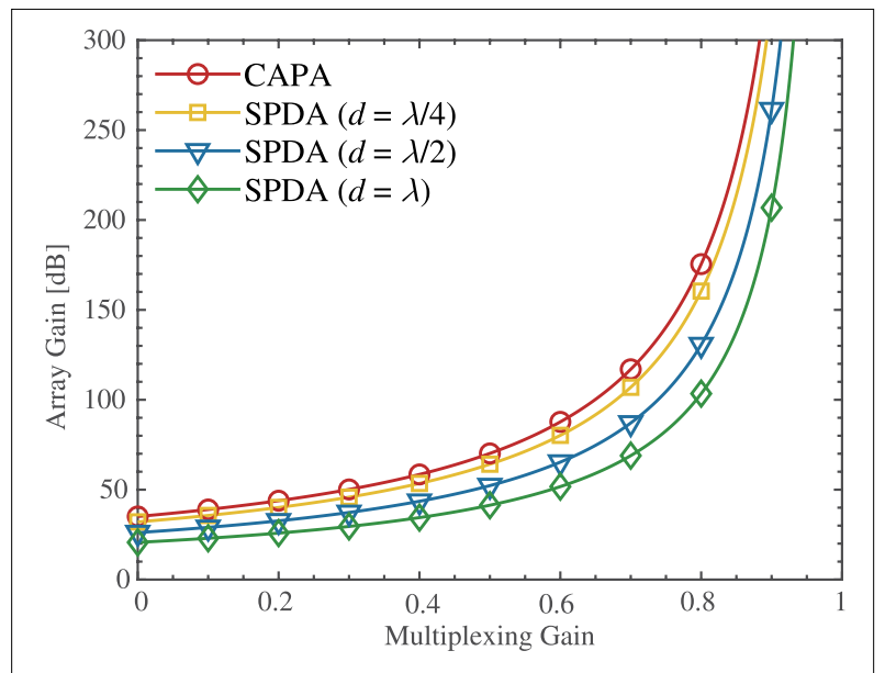
FIGURE 3. The trade-off of array gain and multiplexing gain for CAPA and SPDA with different antenna spacing d [4].
