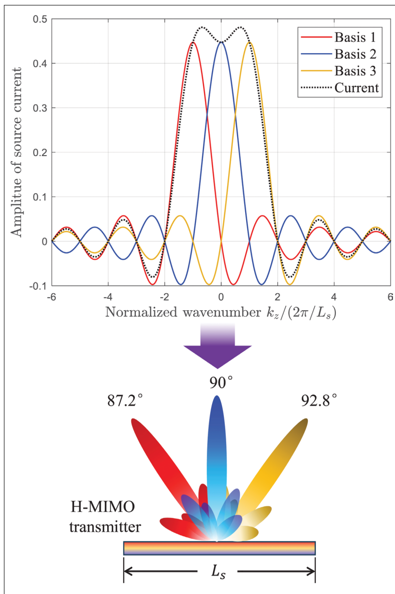
FIGURE 4. An illustration of WDM scheme [11]. The source current is composed of three nearly orthogonal basis functions, each carrying one data stream.
